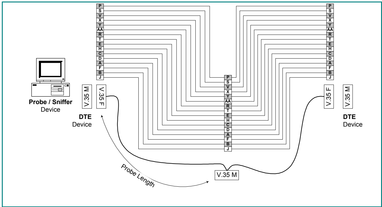
Figure 7 V.35 - Sniffer/WAN Probe 'Y' Cable
